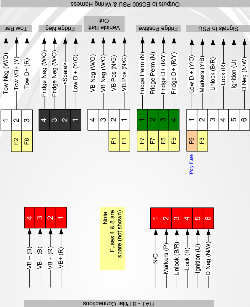
EM40 Interface Connections
