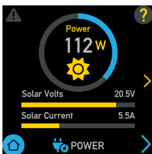
Solar+ additional screen
